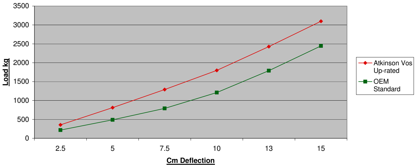
Atkinson Vos HD Springs U1000 - U1650 Rear v Standard Springs Cm & Kg
