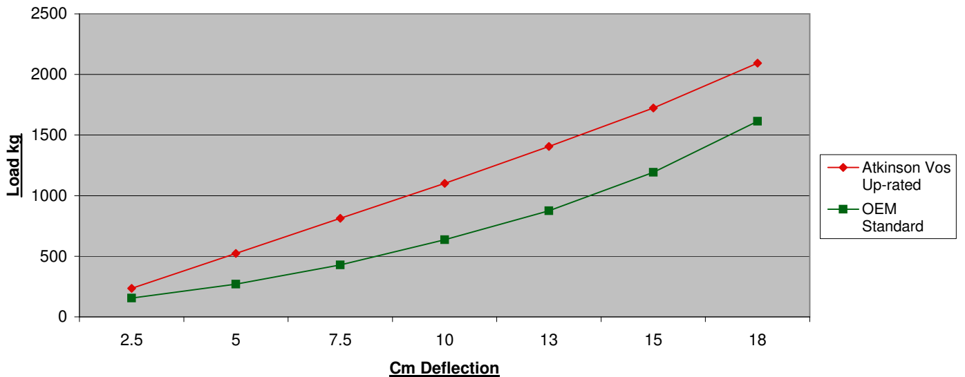
Atkinson Vos HD Springs 408/418 Rear v Standard Springs Cm & Kg
