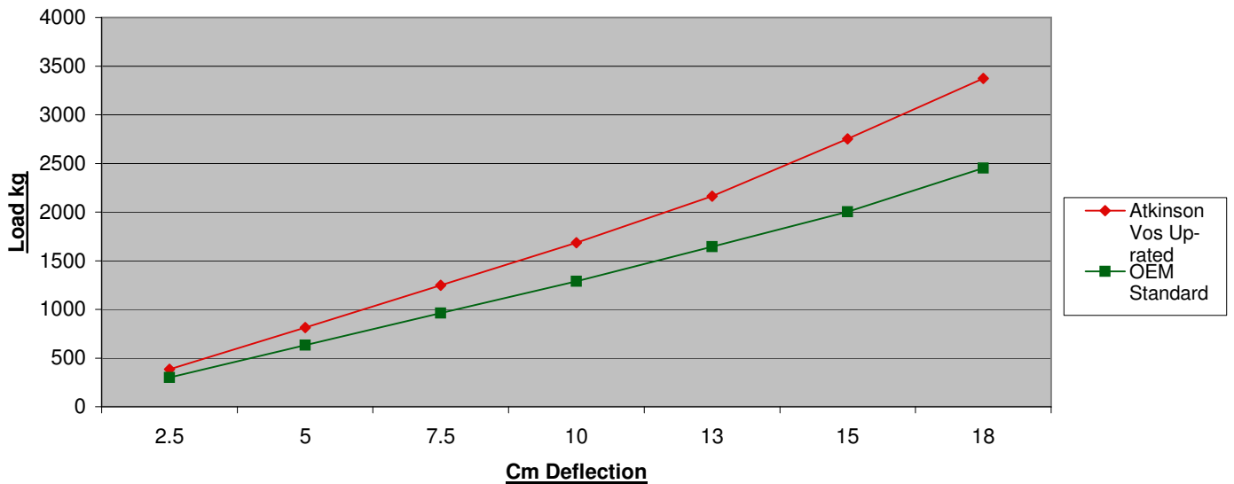
Atkinson Vos HD Springs U1300 - U2450 Front v Standard Springs Cm & Kg
